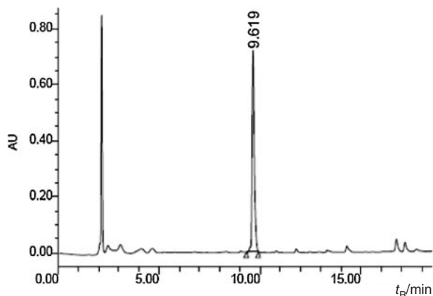
Figure 4. HPLC analysis of the crude sample of TFA·Tyr-Gly-Gly-Phe-Leu-NH 2 ( 15 ). TFFH-Oxyrna is used as coupling reagent. Conditions: HPLC system: Linear gradient 20 to 80% CH 3 CN/H 2 O, 0.1% TFA over 30 min, detection at 200 nm Water Symmetry C 18 5 μm 4.6 × 150 mm. t R = 9.619 min (98.3%).
