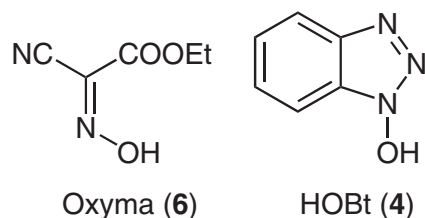
Figure 2. Structure of Oxyima (6) and HOBt (4).
