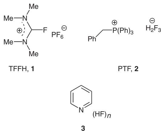
Figure 1. Structures of fluorinating reagents.
